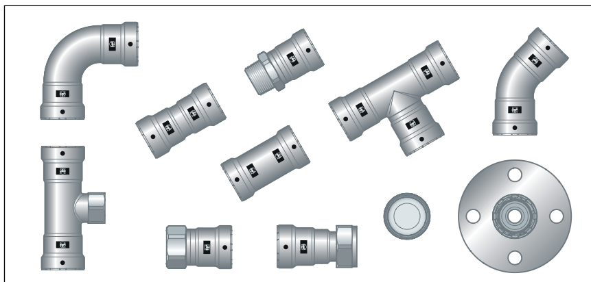
Fig. 2: Megapress press connectors
