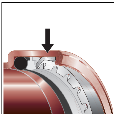
Fig. 6: Cutting ring
